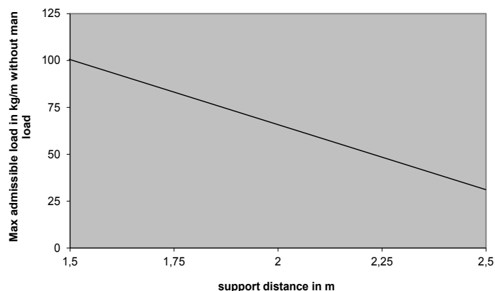
LOADING GRAPH Thks. 0,6 mm
