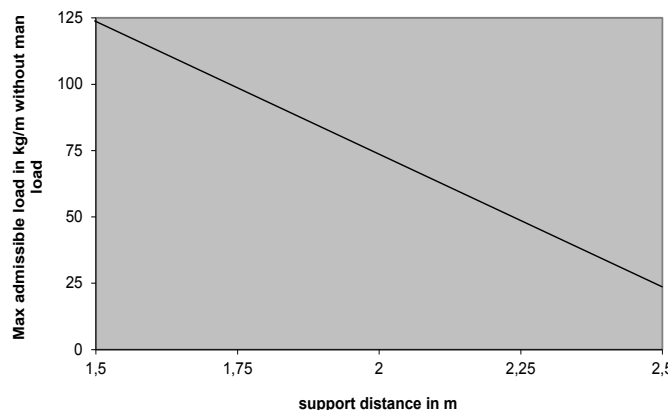
LOADING GRAPH Thks. 1,0 mm
