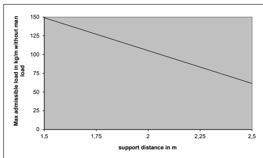
LOADING GRAPH Thks. 1,25 mm
