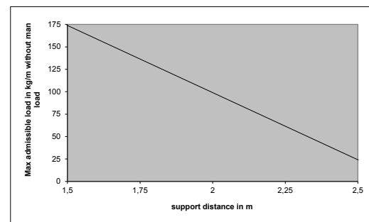
LOADING GRAPH Thks. 1,5 mm
